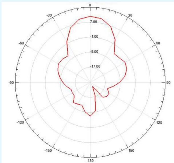
H Plane Radiation Pattern
